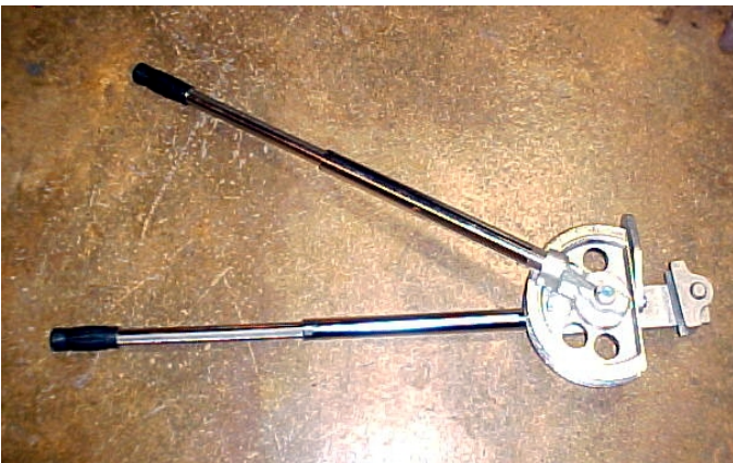
Imperial 1" OD Tubing Bender 3.5" radius For copper and aluminum
